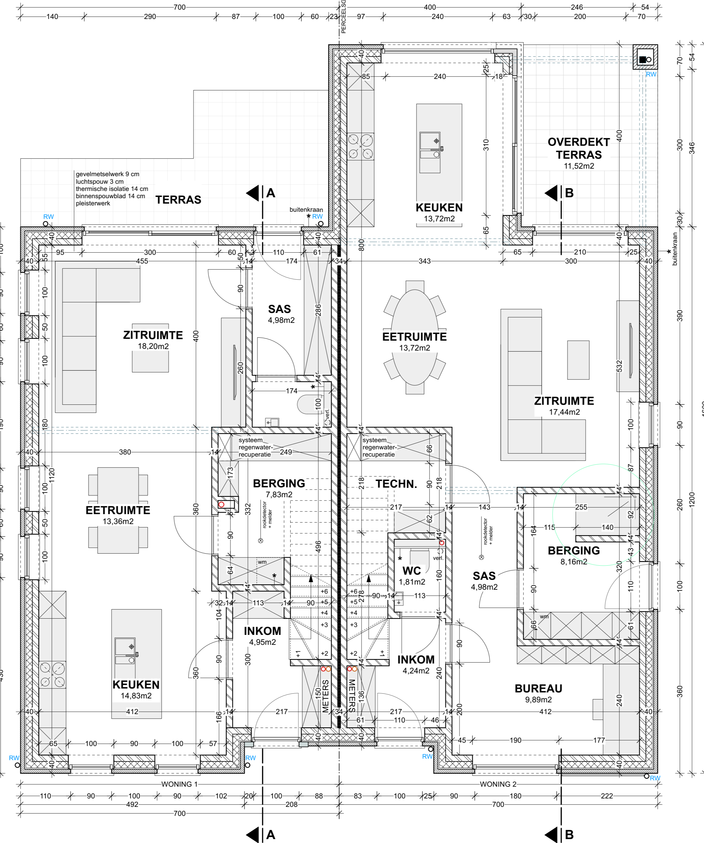
GRONDPLAN WONING 1 & 2 bruto opp. giv woning 1: 82,76m 2 bruto opp. giv woning 2: 97,75m 2
